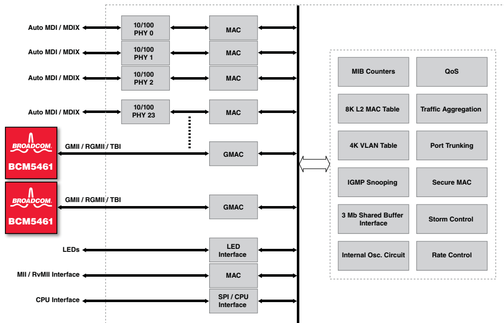
BCM5324M Block Diagram
