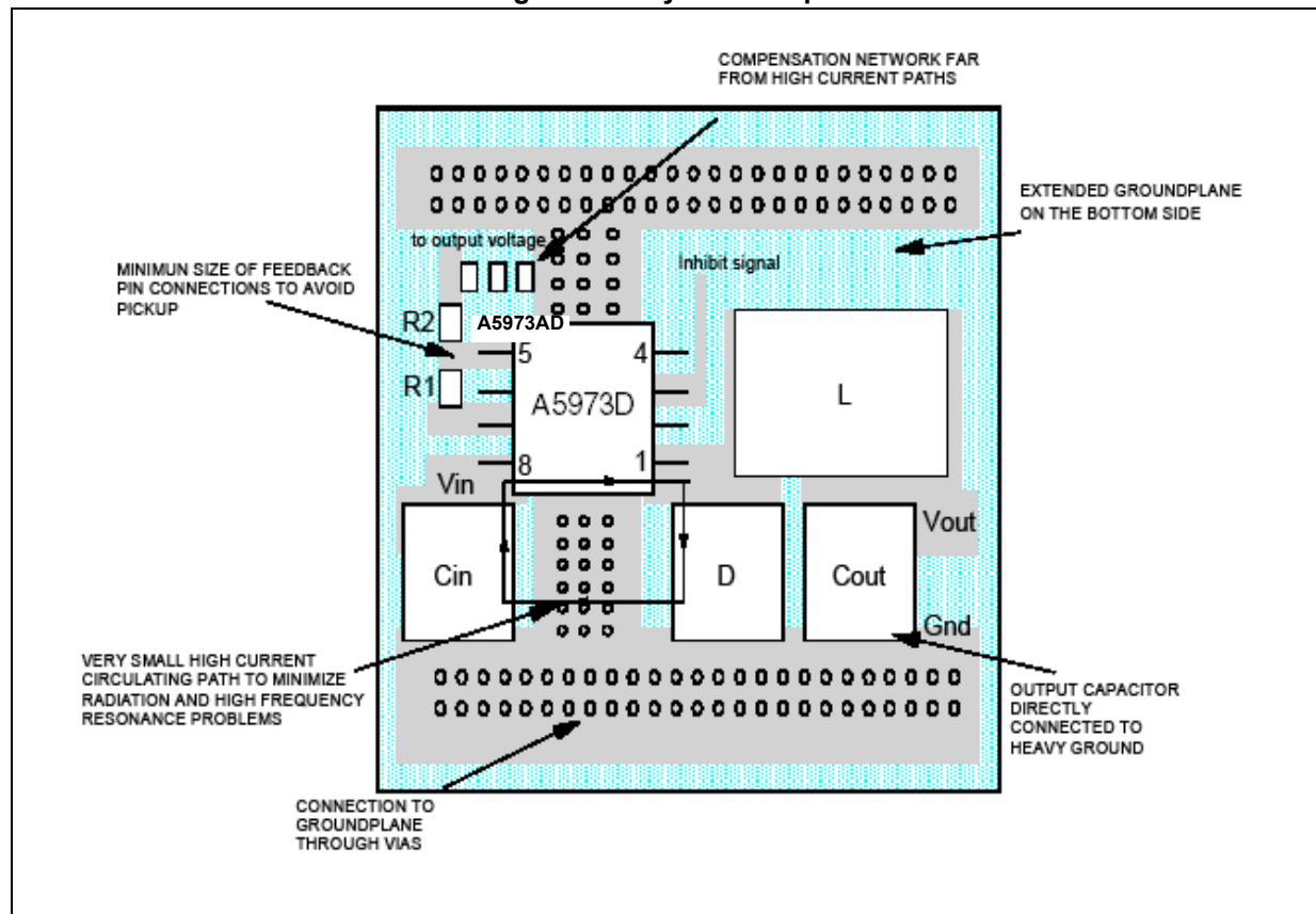
Figure 13. Layout example
