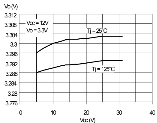
Figure 30. Line regulation
