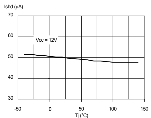
Figure 32. Shutdown current vs. junction temperature
