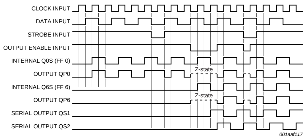
Fig 7. Timing diagram
