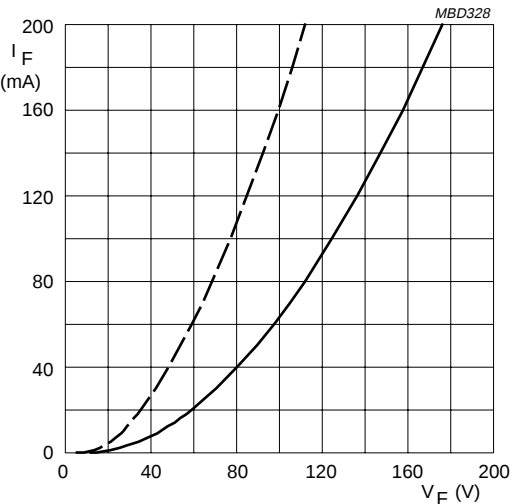
BY9318. Dotted line: T_J = 120\text{ }^{\circ}\text{C} . Solid line: T_J = 25\text{ }^{\circ}\text{C} .
