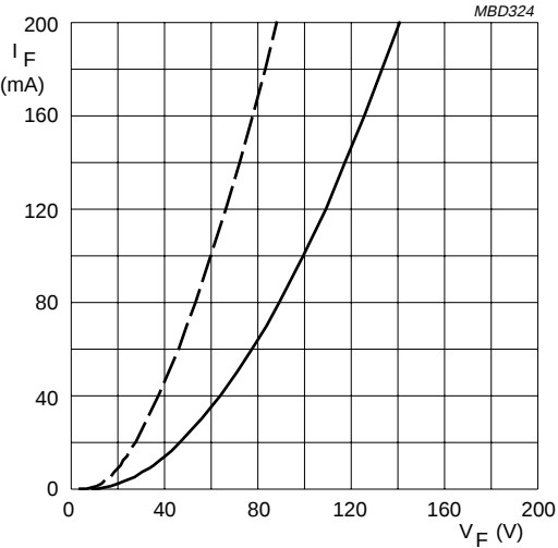
BY9314. Dotted line: T_J = 120\text{ }^{\circ}\text{C} . Solid line: T_J = 25\text{ }^{\circ}\text{C} .
