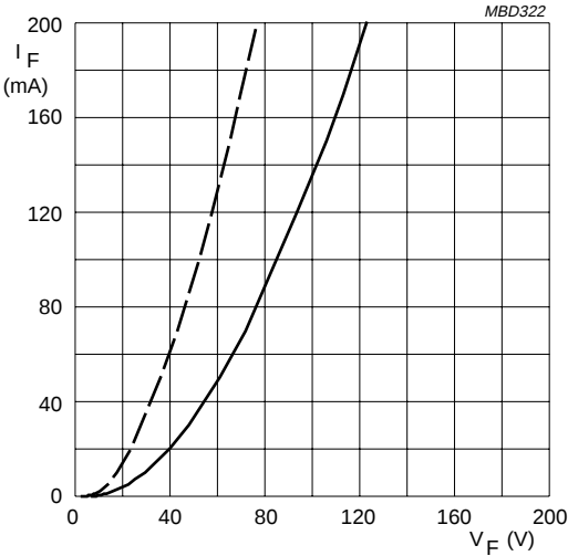
BY9312. Dotted line: T_J = 120\text{ }^{\circ}\text{C} . Solid line: T_J = 25\text{ }^{\circ}\text{C} .
