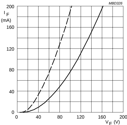
BY9316. Dotted line: T_J = 120\text{ }^{\circ}\text{C} . Solid line: T_J = 25\text{ }^{\circ}\text{C} .
