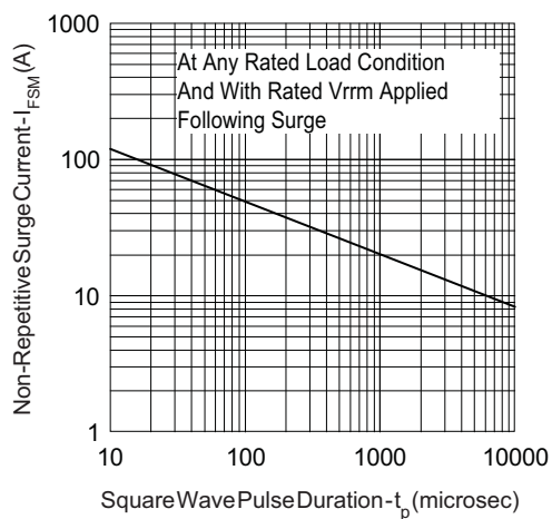
Fig. 6 - Maximum Non-Replicative Surge Current (Per Leg)
