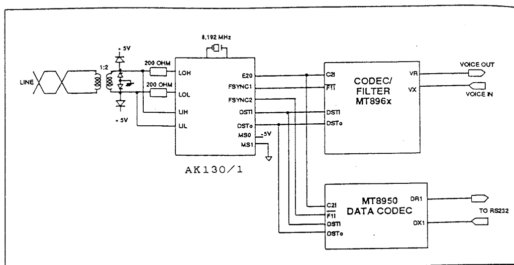
Fig-11 Typical Application - Data and Voice Terminal
