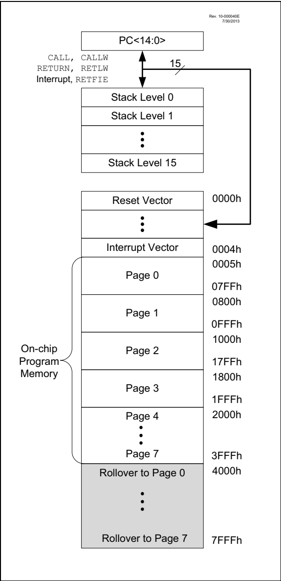
FIGURE 3-2: PROGRAM MEMORY MAP AND STACK FOR PIC16(L)F1716
