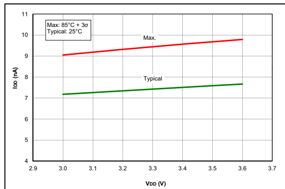
FIGURE 35-39: I_{DD} , Brown-out Reset (BOR), BORV = 1 , PIC16LF1713/6 Only.
