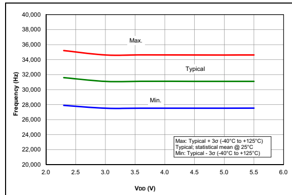
FIGURE 35-58: LFINTOSC Frequency, PIC16F1713/6 Only.
