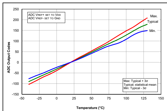
FIGURE 35-89: Temp. Indicator Slope Normalized to 20^\circ C , High Range, V_{DD} = 3.0V , PIC16F1713/6 Only.
