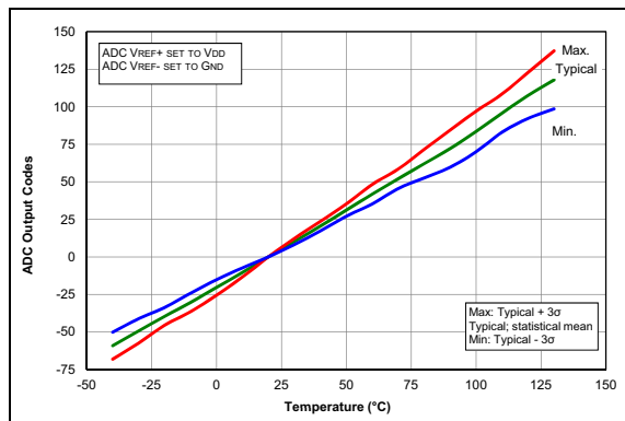
FIGURE 35-88: Temp. Indicator Slope Normalized to 20^\circ C , High Range, V_{DD} = 5.5V , PIC16F1713/6 Only.
