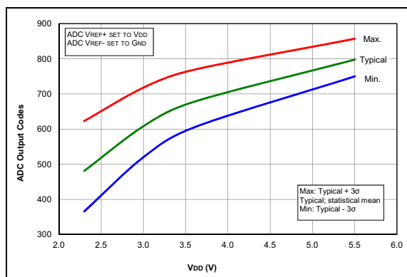
FIGURE 35-86: Temp. Indicator Initial Offset, Low Range, Temp. = 20^\circ C , PIC16F1713/6 Only.
