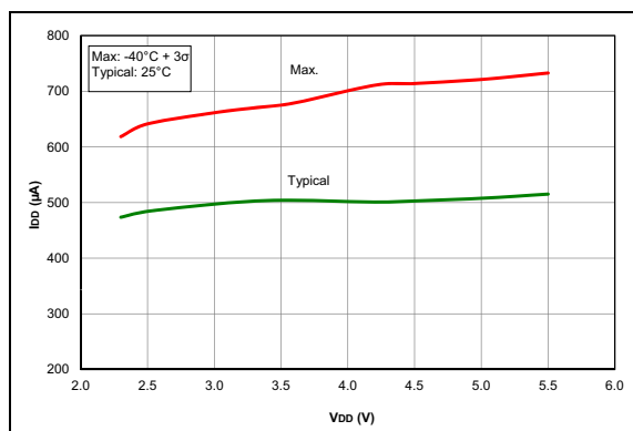
FIGURE 35-50: I_D , Comparator, NP Mode ( C_{XSP} = 1 ), PIC16F1713/6 Only.
