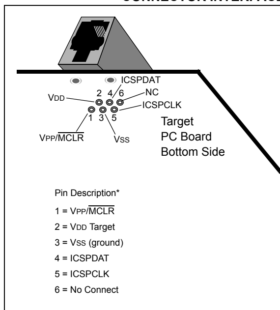
FIGURE 32-1: ICD RJ-11 STYLE CONNECTOR INTERFACE
