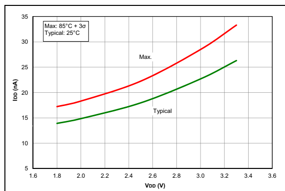
FIGURE 35-37: I_{DD} , Fixed Voltage Reference (FVR), PIC16LF1713/6 Only.
