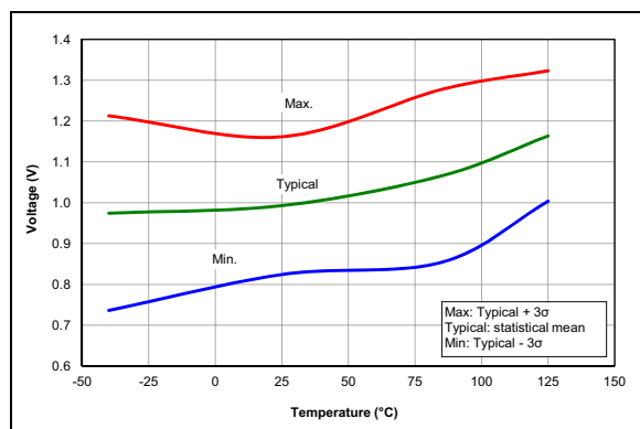
FIGURE 35-73: POR Rearm Voltage, NP Mode, PIC16LF1713/6 Only.
