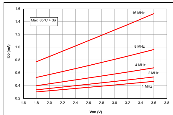
FIGURE 35-24: I_{DD} Maximum, HFINTOSC Mode, PIC16LF1713/6 Only.
