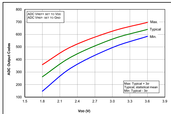
FIGURE 35-87: Temp. Indicator Initial Offset, Low Range, Temp. = 20^\circ C , PIC16LF1713/6 Only.
