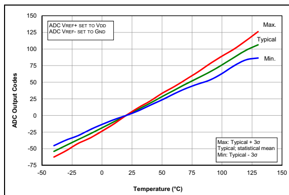
FIGURE 35-90: Temp. Indicator Slope Normalized to 20^\circ C , Low Range, V_{DD} = 3.0V , PIC16F1713/6 Only.
