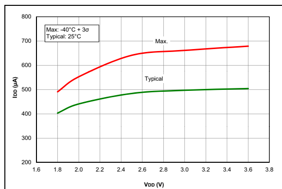
FIGURE 35-49: I_D , Comparator, NP Mode ( C_{XSP} = 1 ), PIC16LF1713/6 Only.
