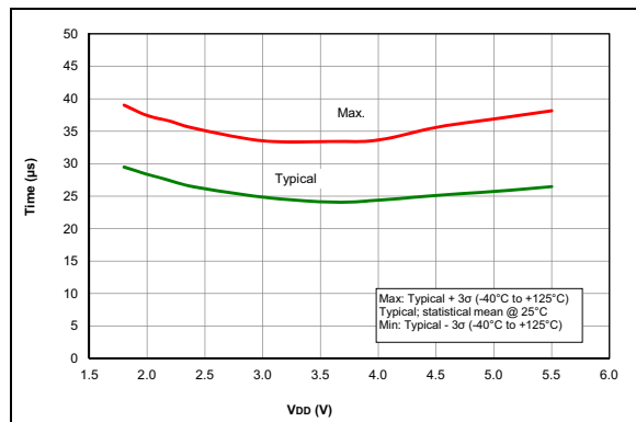
FIGURE 35-75: Wake From Sleep, V_{REGPM} = 1 .
