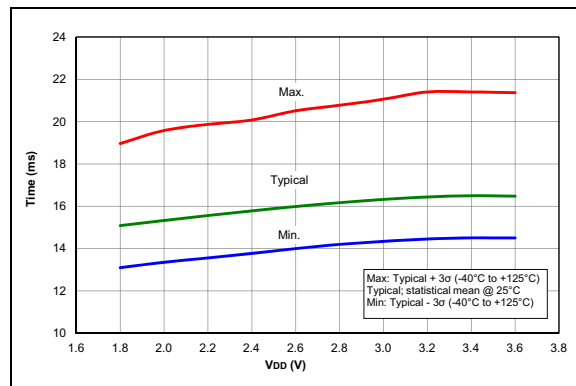
FIGURE 35-60: WDT Time-Out Period, PIC16LF1713/6 Only.
