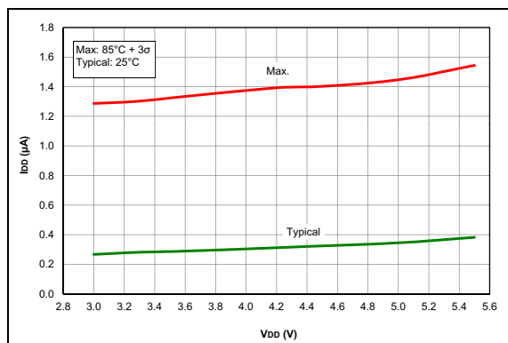
FIGURE 35-42: I_{DD} , LP Brown-out Reset ( LPBOR = 0 ), PIC16F1713/6 Only.
