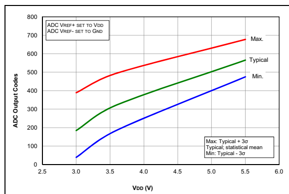
FIGURE 35-85: Temp. Indicator Initial Offset, High Range, Temp. = 20^\circ C , PIC16F1713/6 Only.
