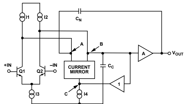
Figure 33. AD797 Block Diagram
