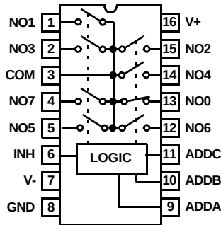
ISL84051 (SOIC, SSOP) TOP VIEW
