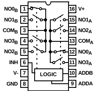
ISL84052 (SOIC, SSOP) TOP VIEW
