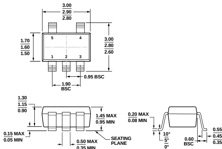
Figure 22. 5-Lead Small Outline Transistor Package [SOT-23]
