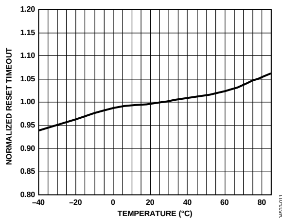
Figure 12. Normalized Reset Timeout Period vs. Temperature
