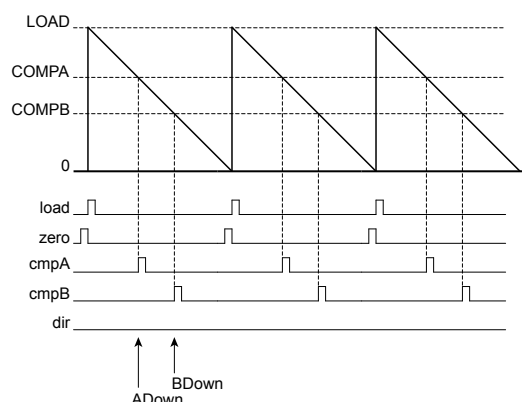
Figure 22-3. PWM Count-Down Mode
