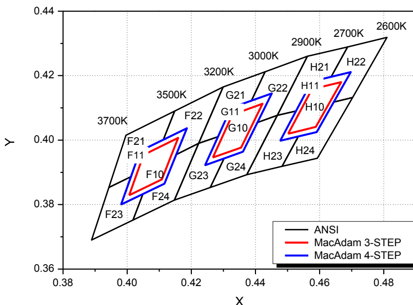
CIE Chromaticity Diagram, T_j=25^{\circ}\text{C} , I_F=1.1\text{A}
