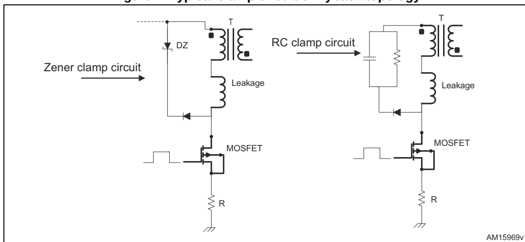
Figure 7. Typical clamp circuit of flyback topology
