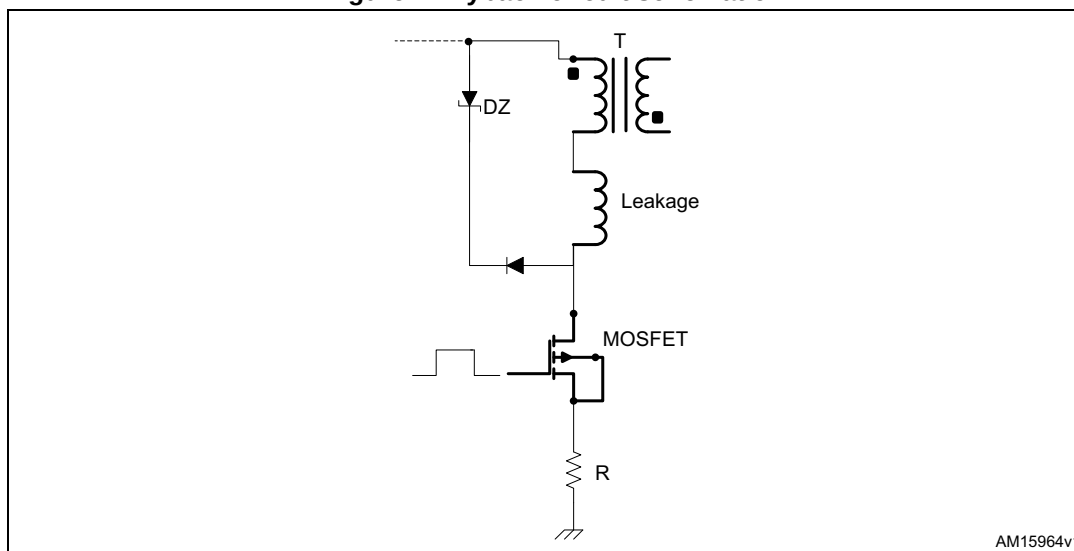
Figure 2. Flyback circuit schematic
