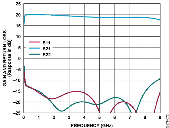
Figure 72. Gain and Return Loss vs. Frequency, 1 MHz to 9 GHz, V_{DD} = 5 V, I_{DQ} = 95 mA
