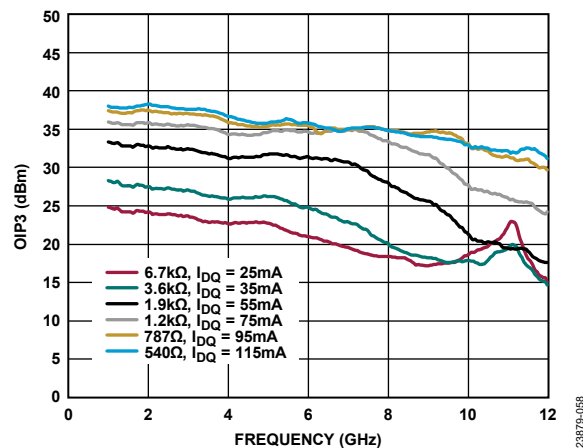
Figure 58. OIP3 vs. Frequency for Various Bias Resistor Values and I_{DQ} , 1 GHz to 12 GHz, V_{DD} = 5 V
