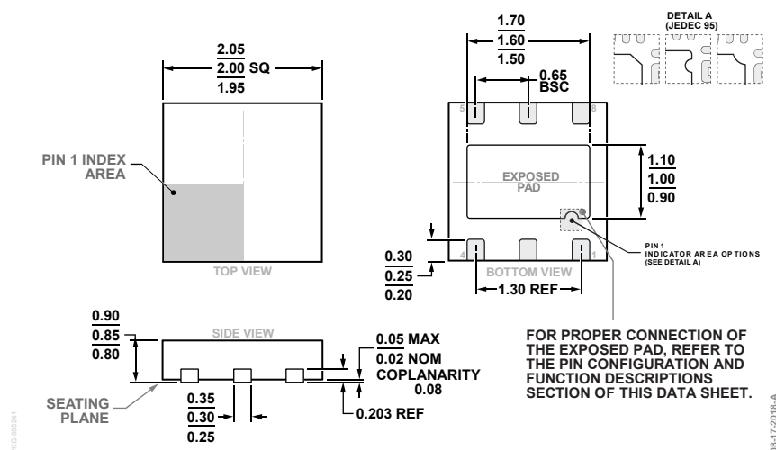
Figure 76. 6-Lead Lead Frame Chip Scale Package [LFCSP] 2 mm x 2 mm Body and 0.85 mm Package Height (CP-6-12)
