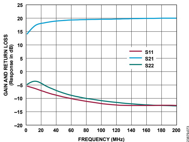
Figure 73. Gain and Return Loss vs. Frequency, 1 MHz to 200 MHz, V_{DD} = 5 V, I_{DQ} = 95 mA
