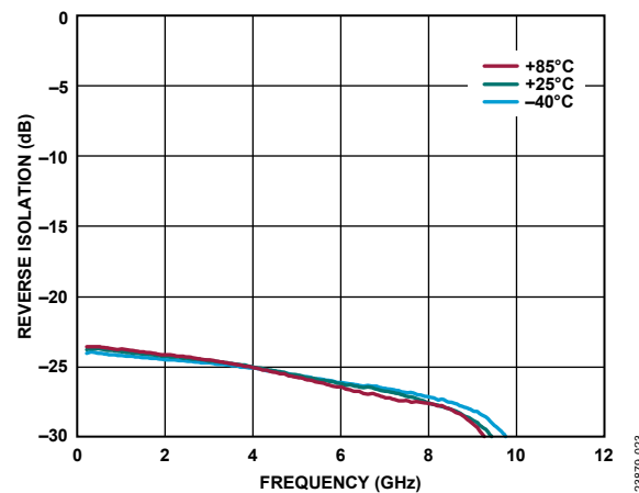
Figure 23. Reverse Isolation vs. Frequency for Various Temperatures, 200 MHz to 12 GHz, V_{DD} = 5 V , I_{DQ} = 95 mA
