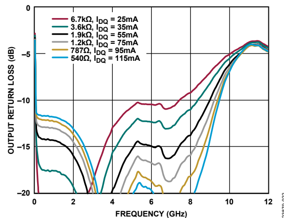
Figure 22. Output Return Loss vs. Frequency for Various Bias Resistor Values and I_{DQ} , V_{DD} = 5 V
