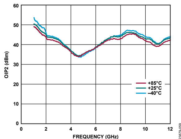
Figure 59. OIP2 vs. Frequency for Various Temperatures, 1 GHz to 12 GHz, V_{DD} = 5 V, I_{DQ} = 95 mA
