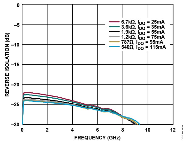
Figure 24. Reverse Isolation vs. Frequency for Various Bias Resistor Values and I_{DQ} , V_{DD} = 5 V
