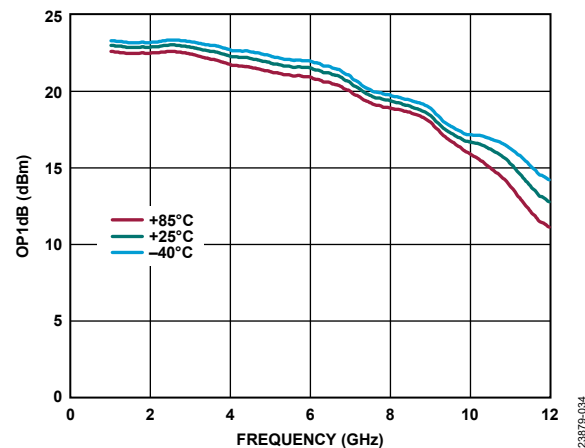
Figure 34. OP1dB vs. Frequency for Various Temperatures, 1 GHz to 12 GHz, V_{DD} = 5\text{ V} , I_{DQ} = 95\text{ mA}
