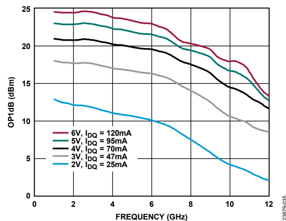
Figure 35. OP1dB vs. Frequency for Various Supply Voltages and I_{DQ} , 1 GHz to 12 GHz, R_{BIAS} = 787\ \Omega
