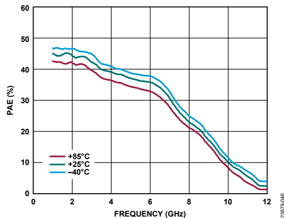
Figure 46. PAE vs. Frequency for Various Temperatures, 1 GHz to 12 GHz, V_{DD} = 5\text{ V} , I_{DQ} = 95\text{ mA}
