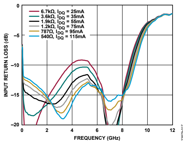
Figure 17. Input Return Loss vs. Frequency for Various Bias Resistor Values and I_{DQ} , V_{DD} = 5\text{ V}
