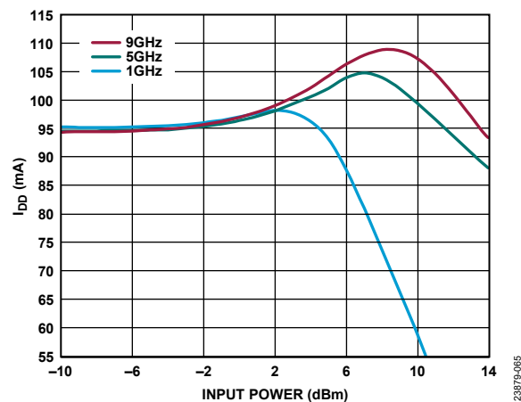
Figure 65. I_{DD} vs. Input Power for Various Frequencies, V_{DD} = 5 V
