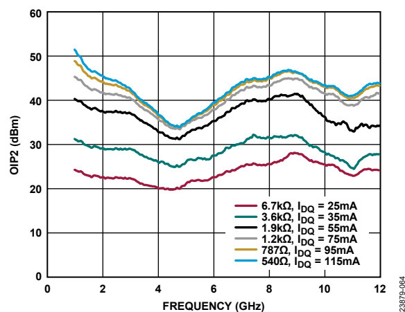
Figure 64. OIP2 vs. Frequency for Various Bias Resistor Values and I_{DQ} , 1 GHz to 12 GHz, V_{DD} = 5 V
