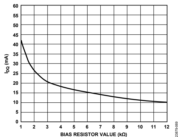
Figure 69. I_{DQ} vs. Bias Resistor Value, 1 k \Omega to 12 k \Omega , V_{DD} = 3 V
