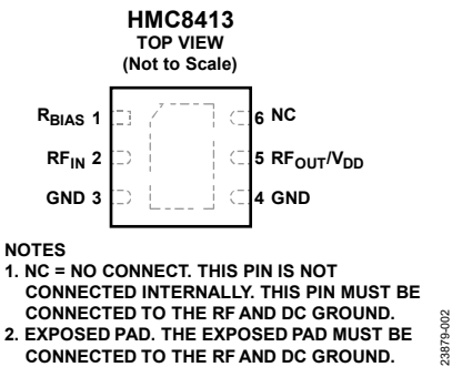
Figure 2. Pin Configuration
