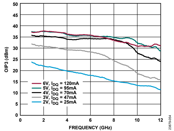
Figure 54. OIP3 vs. Frequency for Various Supply Voltages and I_{DQ} , 1 GHz to 12 GHz, R_{BIAS} = 787 \Omega
