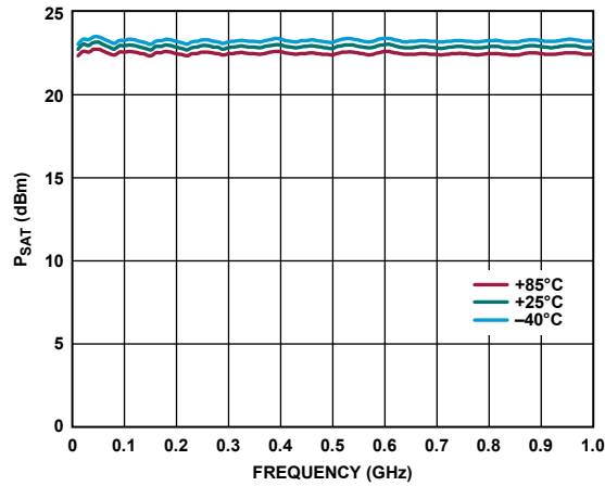
Figure 37. P_{SAT} vs. Frequency for Various Temperatures, 0.01 GHz to 1.0 GHz, V_{DD} = 5\text{ V} , I_{DQ} = 95\text{ mA}
