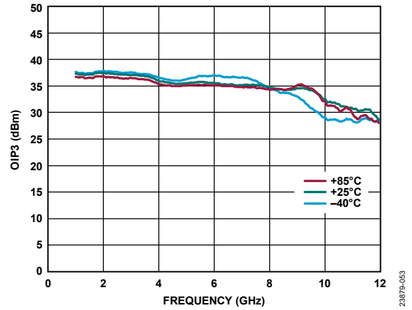
Figure 53. OIP3 vs. Frequency for Various Temperatures, 1 GHz to 12 GHz, V_{DD} = 5 V , I_{DQ} = 95 mA
