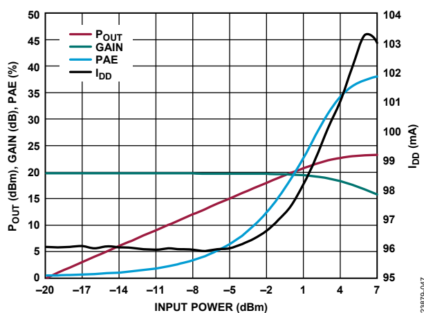
Figure 47. P_{OUT} , Gain, PAE, and I_{DD} vs. Input Power, Power Compression at 5 GHz, V_{DD} = 5\text{ V} , R_{BIAS} = 787\ \Omega
