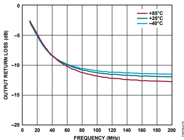
Figure 15. Output Return Loss vs. Frequency for Various Temperatures, 10 MHz to 200 MHz, V_{DD} = 5\text{ V} , I_{DQ} = 95\text{ mA}
