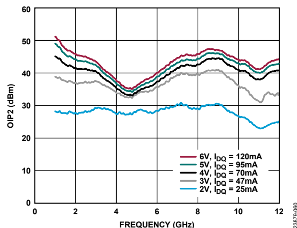
Figure 60. OIP2 vs. Frequency for Various Supply Voltages and I_{DQ} , 1 GHz to 12 GHz, R_{BIAS} = 787 Ω
