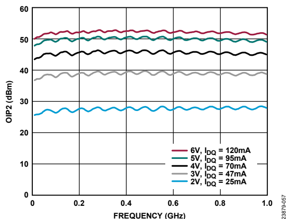
Figure 57. OIP2 vs. Frequency for Various Supply Voltages and I_{DQ} , 0.01 GHz to 1.0 GHz, R_{BIAS} = 787 Ω
