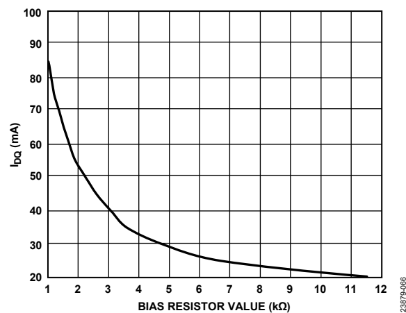
Figure 66. I_{DQ} vs. Bias Resistor Value, 1 k \Omega to 12 k \Omega , V_{DD} = 5 V
