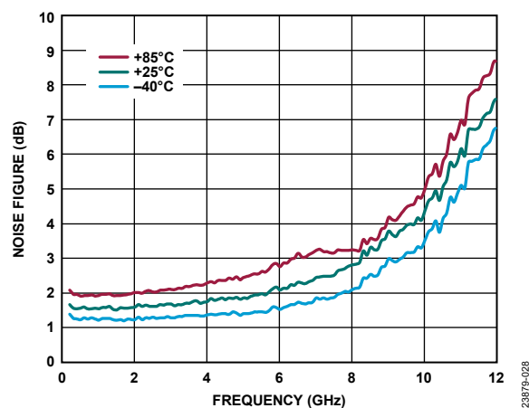
Figure 28. Noise Figure vs. Frequency for Various Temperatures, 200 MHz to 12 GHz, V_{DD} = 5\text{ V} , I_{DQ} = 95\text{ mA}
