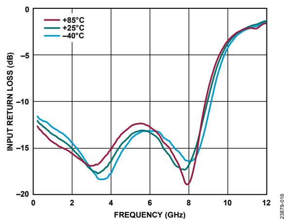
Figure 16. Input Return Loss vs. Frequency for Various Temperatures, 200 MHz to 12 GHz, V_{DD} = 5\text{ V} , I_{DQ} = 95\text{ mA}
