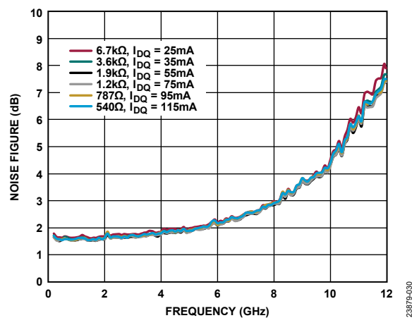
Figure 30. Noise Figure vs. Frequency for Various Bias Resistor Values and I_{DQ} , 200 MHz to 12 GHz, V_{DD} = 5\text{ V}
