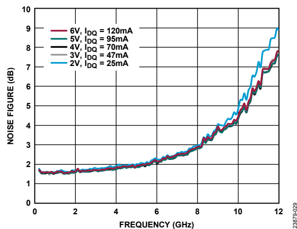
Figure 29. Noise Figure vs. Frequency for Various Supply Voltages and I_{DQ} , 200 MHz to 12 GHz, R_{BIAS} = 787\ \Omega
