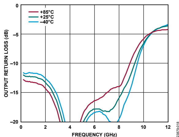
Figure 18. Output Return Loss vs. Frequency for Various Temperatures, 200 MHz to 12 GHz, V_{DD} = 5\text{ V} , I_{DQ} = 95\text{ mA}
