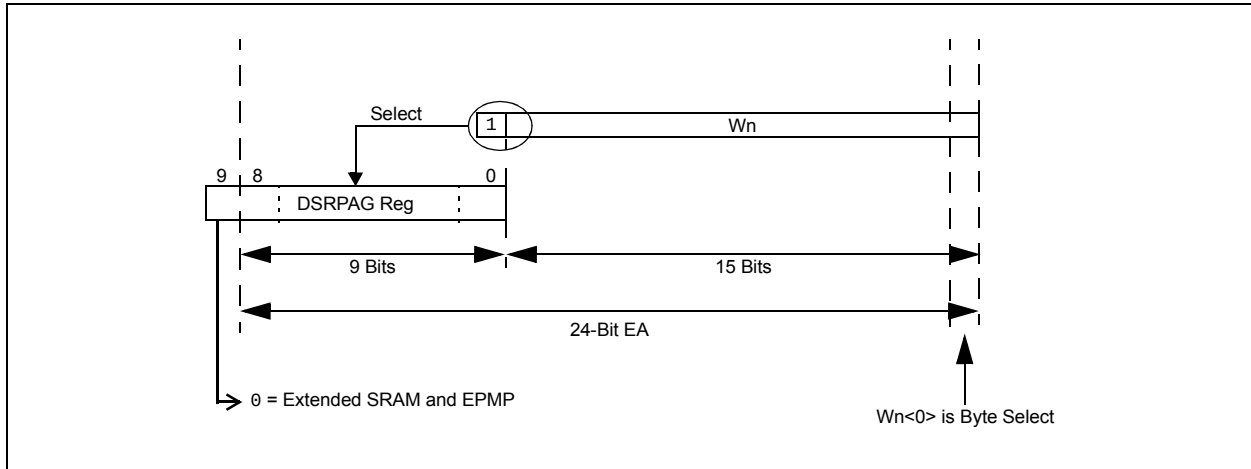
FIGURE 4-5: EDS ADDRESS GENERATION FOR READ OPERATIONS
