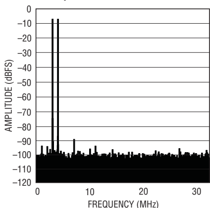
LTC2265-12: 8k Point 2-Tone FFT, f_{IN} = 68\text{MHz} , 69MHz, -1dBFS, 65Mps
