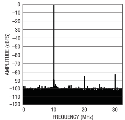
LTC2265-12: 8k Point FFT, f_{IN} = 140\text{MHz} , -1dBFS, 65Mps
