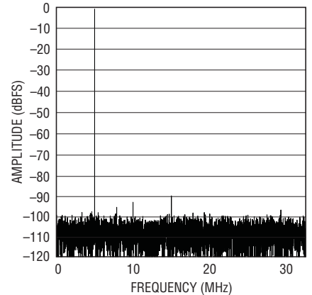
LTC2265-12: 8k Point FFT, f_{IN} = 5\text{MHz} , -1dBFS, 65Mps
