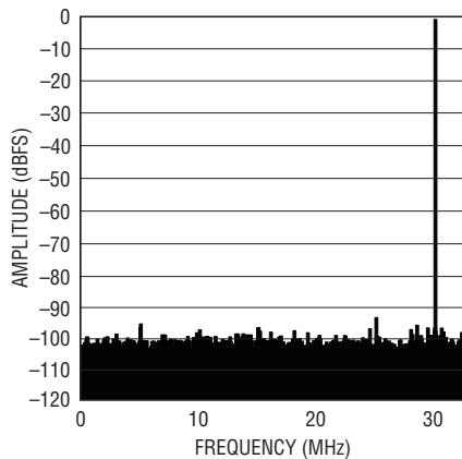
LTC2265-12: 8k Point FFT, f_{IN} = 30\text{MHz} , -1dBFS, 65Mps
