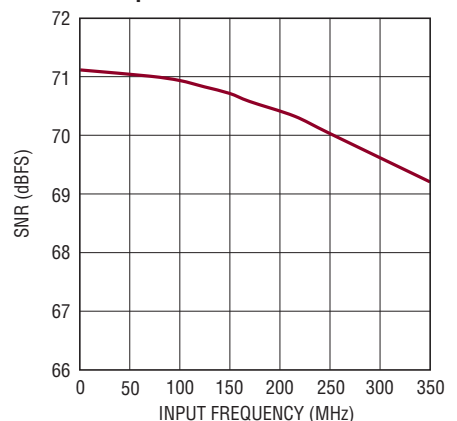
LTC2265-12: SNR vs Input Frequency, -1dBFS, 2V Range, 65Mps
