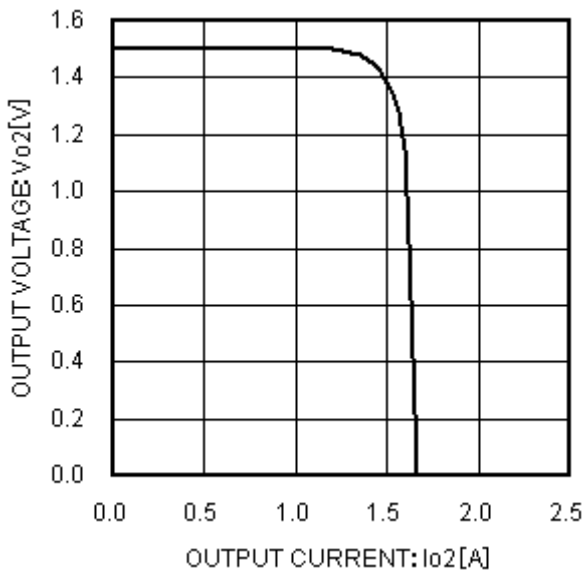
Fig.9 Load Stability (Variable output: 1.5 V)
