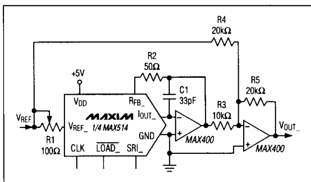
Figure 4. Bipolar Operation for 1/4 of MAX514
