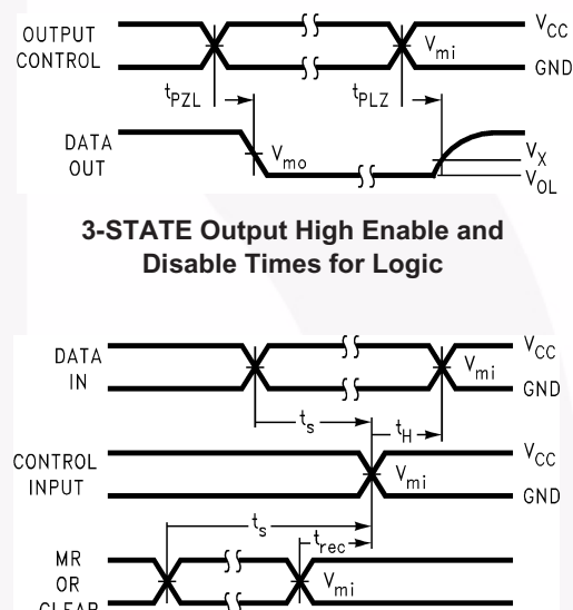
Setup Time, Hold Time and Recovery Time for Logic
