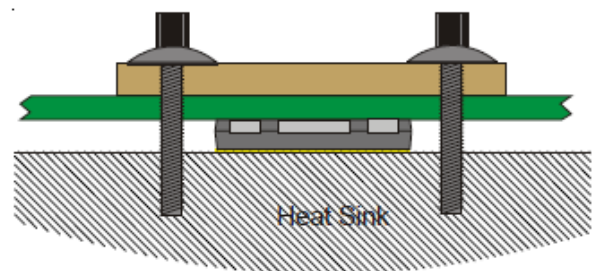
Figure 3– View of IXRFD615X2 mounted in a high-power configuration. For additional device installation instructions see technical note “DE-Series MOSFET Mounting & Installation Instructions” available on the IXYSRF website, www.ixyscolorado.com
