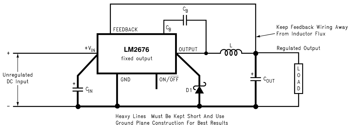
Figure 19. Basic Circuit for Fixed Output Voltage Applications.
