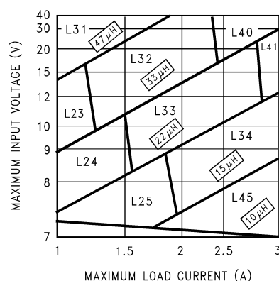
Figure 22. LM2676-5.0
