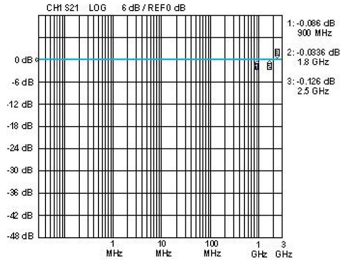
Fig.4 Insertion Loss S21 - I/O to I/O
