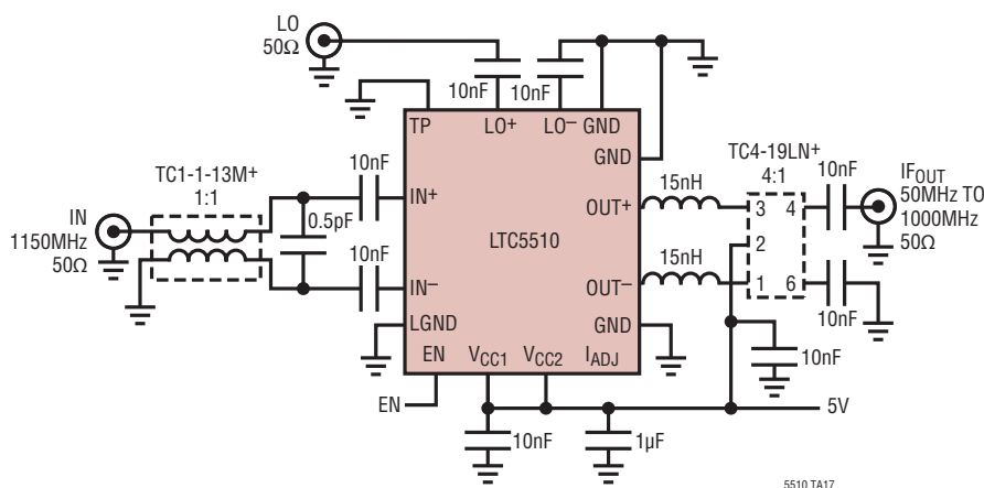
5V CATV Downmixer with 1GHz IF Bandwidth
