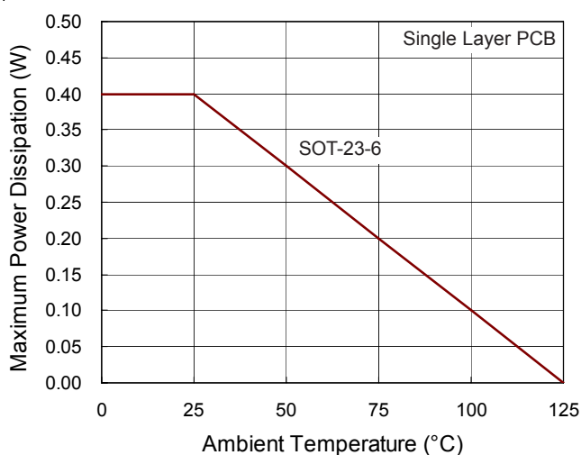
Figure 4. Derating Curves for RT9046 Packages
