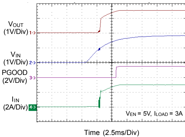
Start Up from V IN
