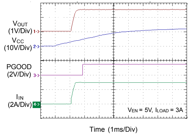
Start Up from V CC
