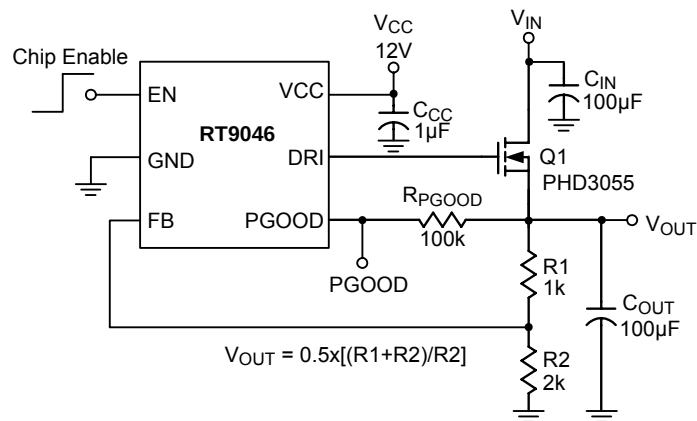
Figure 1. Typical Test Circuit
