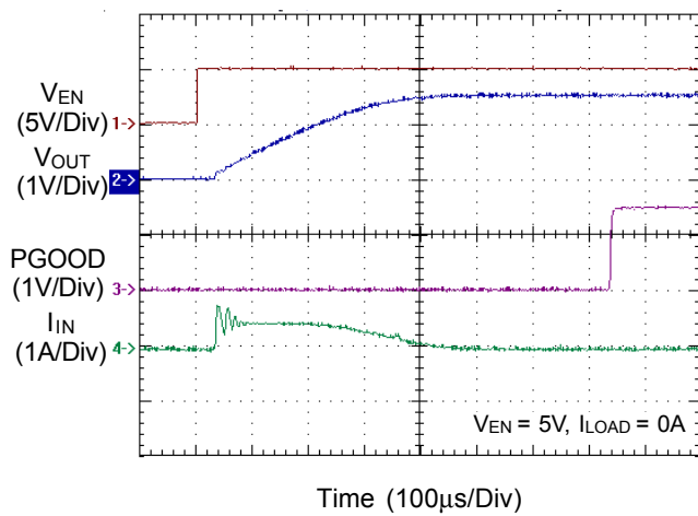
Start Up from EN and Inrush Current
