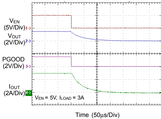
PGOOD Off
