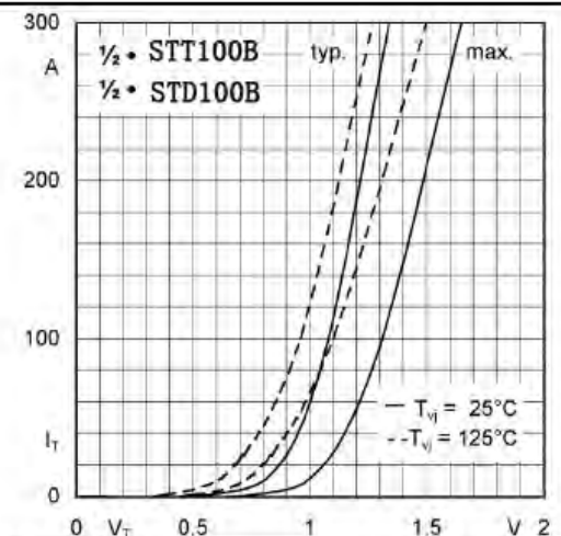
Fig. 7 On-state characteristics
