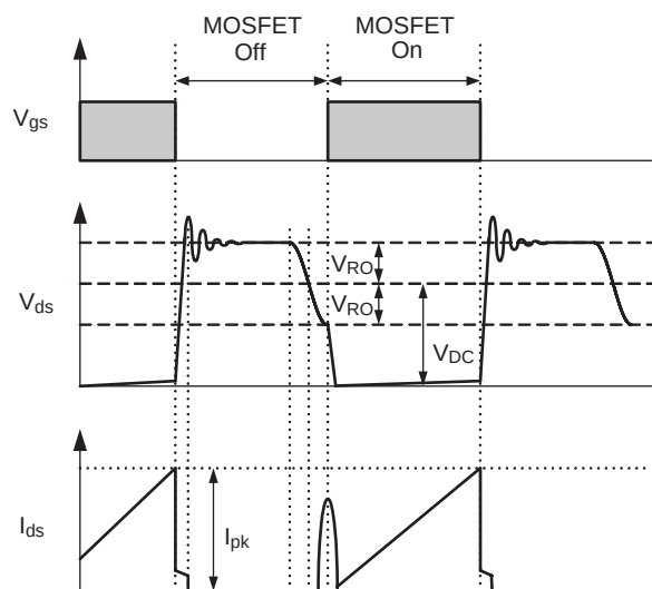
Figure 7. Quasi-Resonant Operation Waveforms
