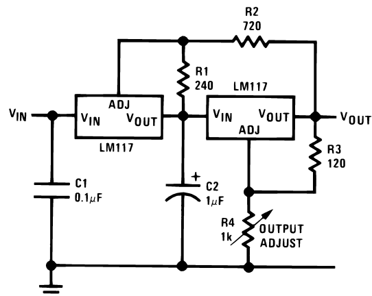
Figure 49. Tracking Preregulator
