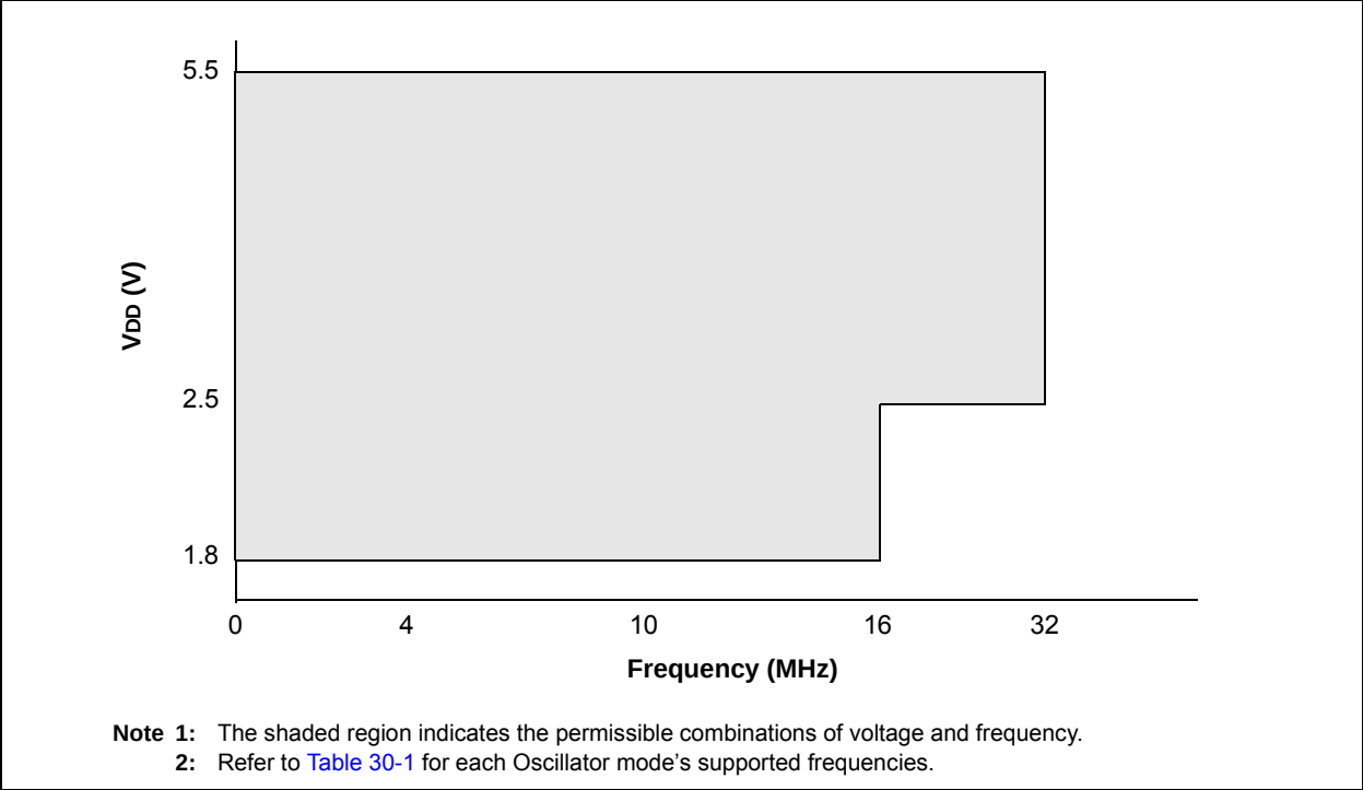
FIGURE 30-1: VOLTAGE FREQUENCY GRAPH, -40°C ≤ TA ≤ +125°C, PIC16F1847 ONLY
