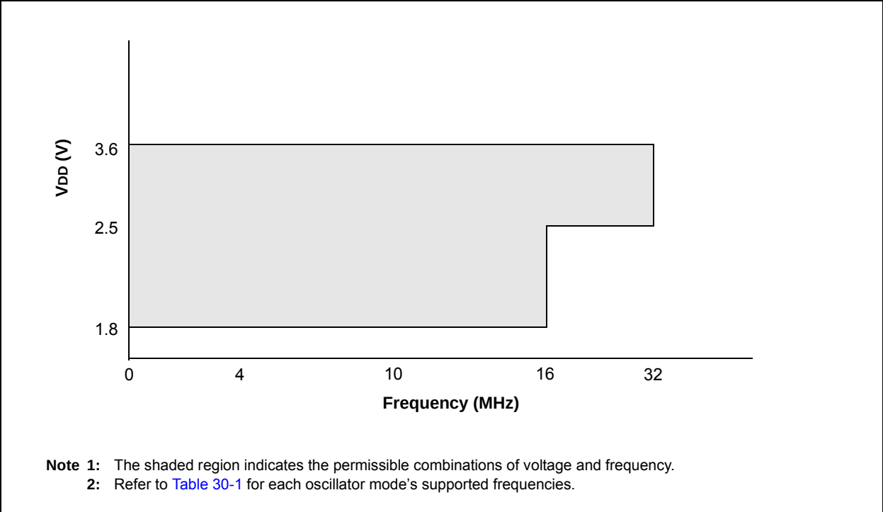
FIGURE 30-2: VOLTAGE FREQUENCY GRAPH, -40°C ≤ TA ≤ +125°C, PIC16LF1847 ONLY
