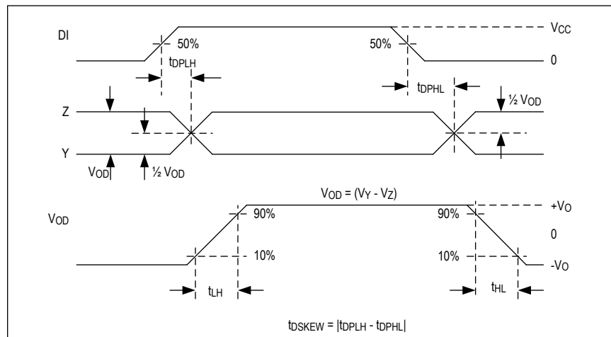
Figure 3. Driver Propagation Delays
