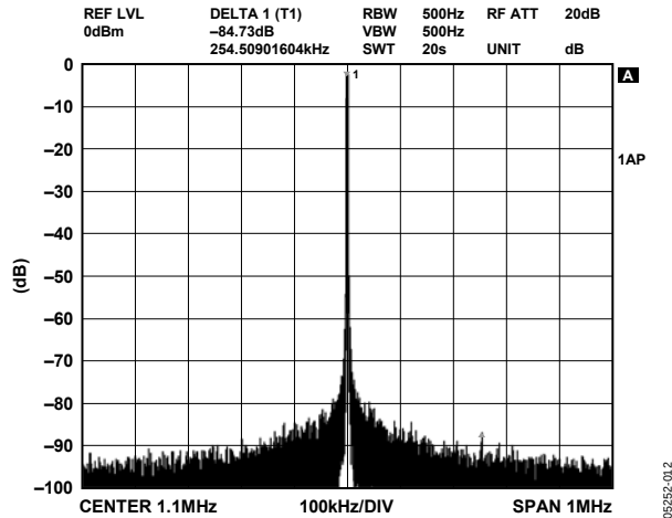
Figure 10. NBSFDR, f_{OUT} = 1.1 MHz, f_{CLK} = 500 MSPS, \pm 1 MHz
