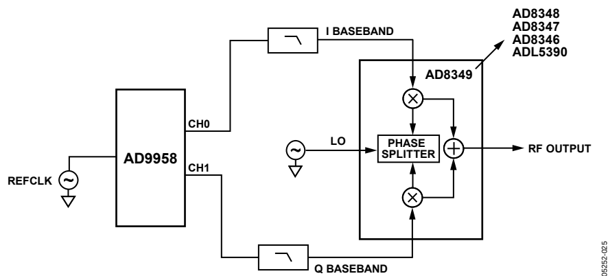
Figure 23. Single-Sideband-Suppressed Carrier Upconversion
