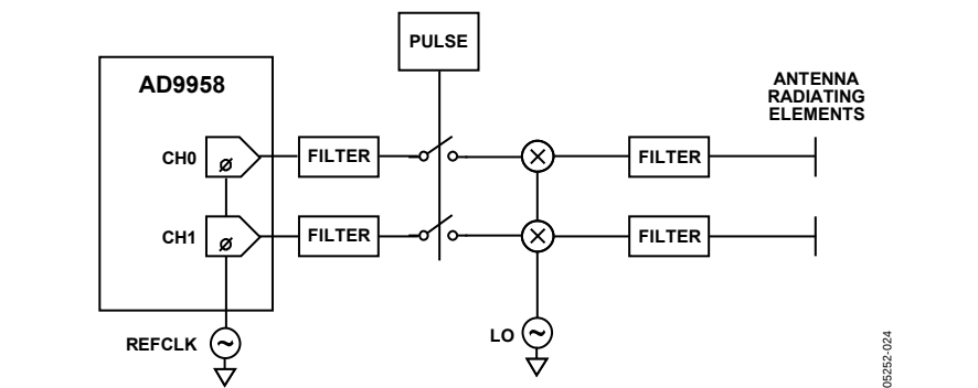
Figure 22. Phase Array Radar Using Precision Frequency/Phase Control from DDS in FMCW or Pulsed Radar Applications; DDS Provides Either Continuous Wave or Frequency Sweep
