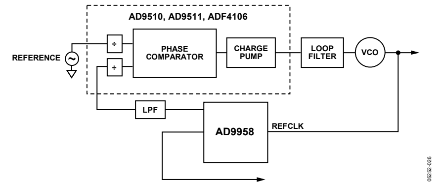
Figure 24. DDS in PLL Locking to Reference Offering Distribution with Fine Frequency and Delay Adjust Tuning
