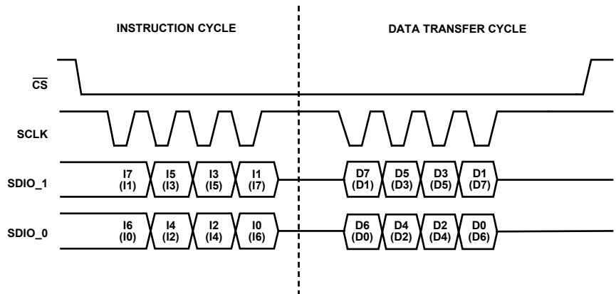
Figure 48. 2-Bit Serial Mode Read Timing—Clock Stall High
