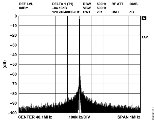
Figure 11. NBSFDR, f_{OUT} = 40.1 MHz, f_{CLK} = 500 MSPS, \pm 1 MHz
