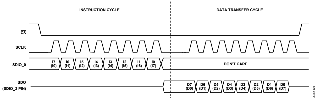
Figure 47. Single-Bit Serial Mode (3-Wire) Read Timing—Clock Stall Low
