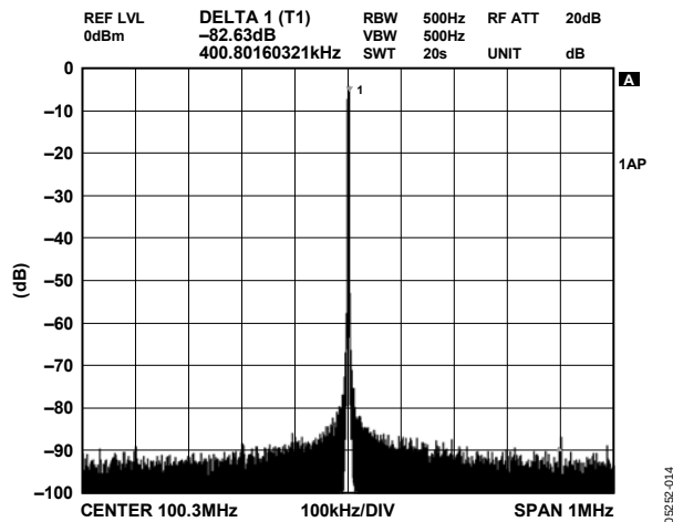
Figure 12. NBSFDR, f_{OUT} = 100.3 MHz, f_{CLK} = 500 MSPS, \pm 1 MHz
