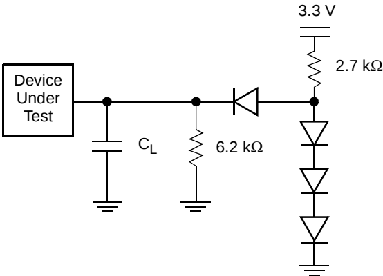
Figure 10. Test Setup
