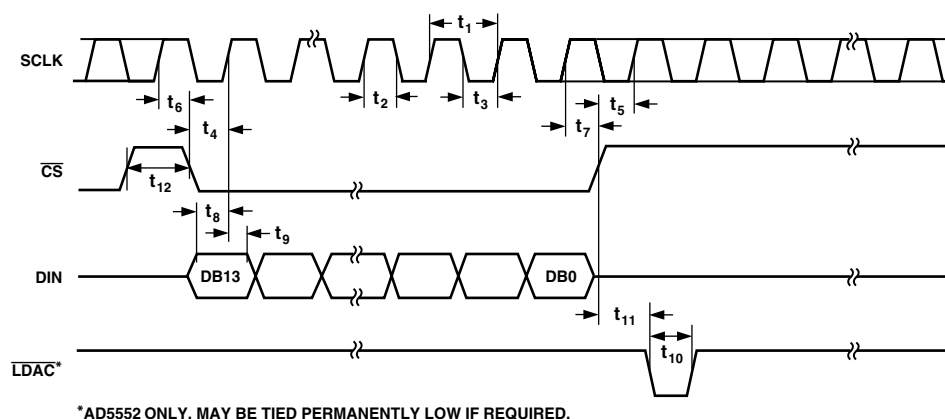
Figure 1. Timing Diagram
