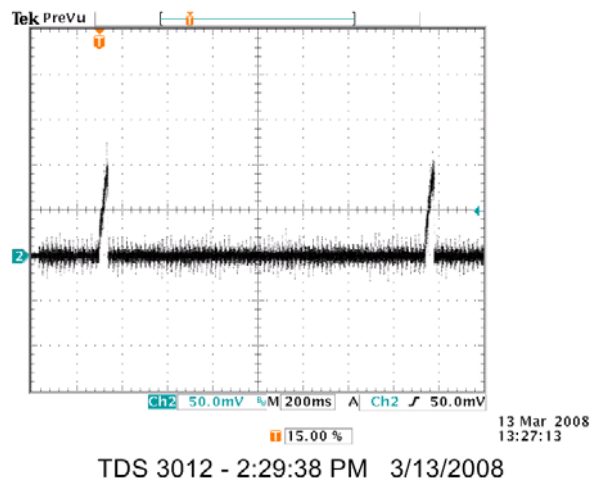
Photo 8: Overload output current, 0.001 Ohm impedance. 24Vin, 50A / div.
