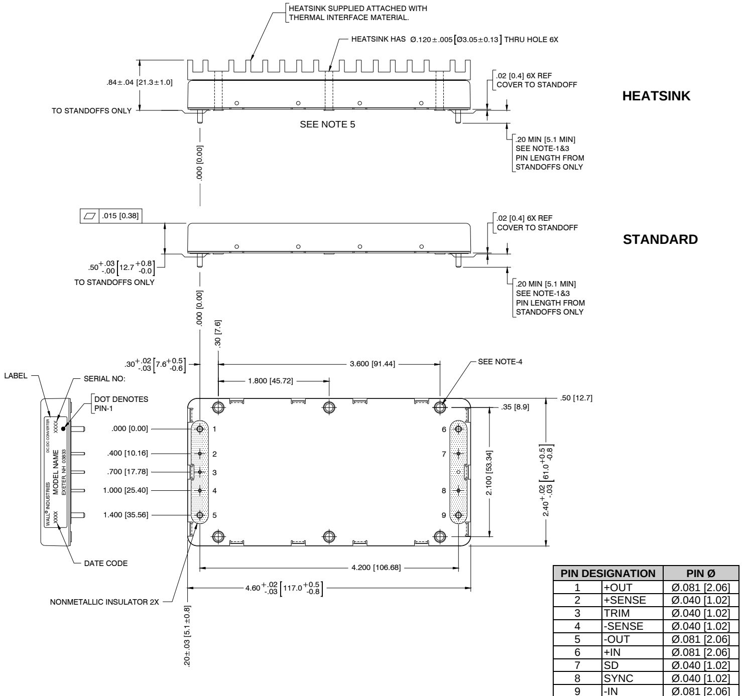
Figure 1: Mechanical Dimensions
