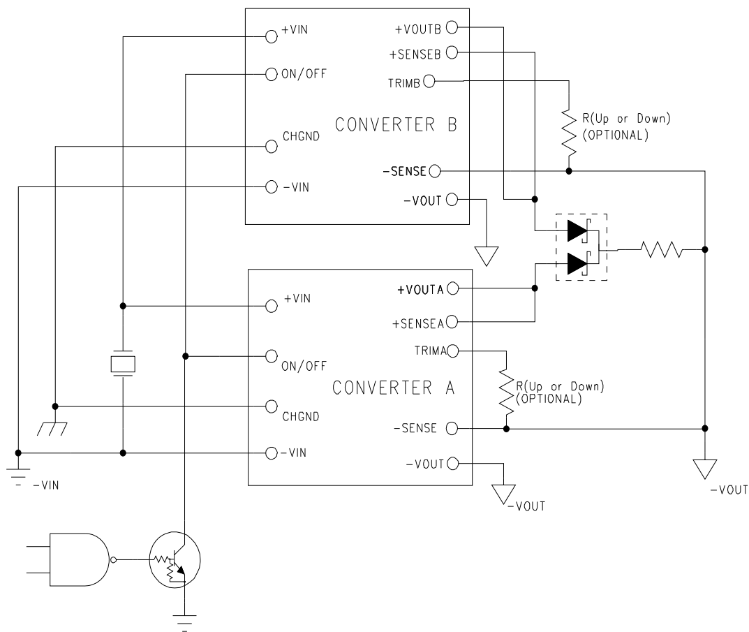
Figure 9: Paralleling Converters
