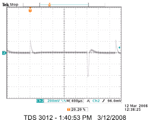
Photo 7: Transient Response 50% to 100% Vin=5V, Iout = 30.0A to 60A @ .2V/ Div Cout=0.1uF Ceramic + 10uF Tantalum
