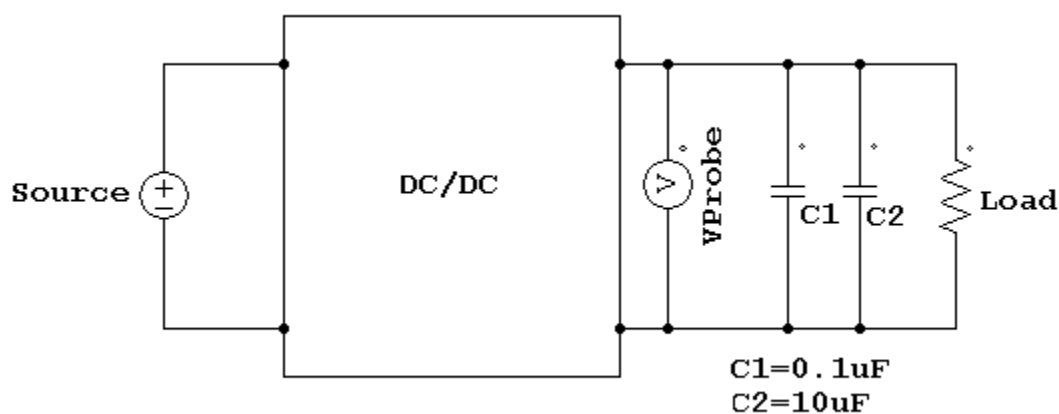
Figure 6: Ripple Voltage Probe Setup
