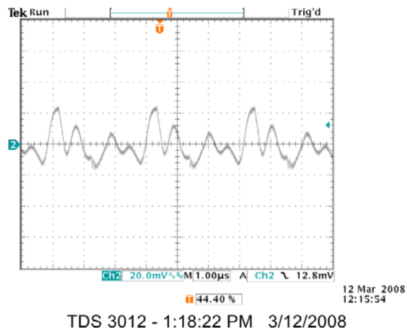
Photo 6: . Output ripple, 36Vin, full load. 20mV / div.
