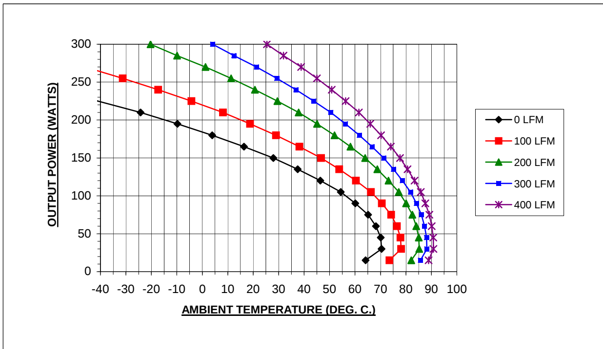
Graph 2: FA12S5-300 Max Ambient vs. Output Power
