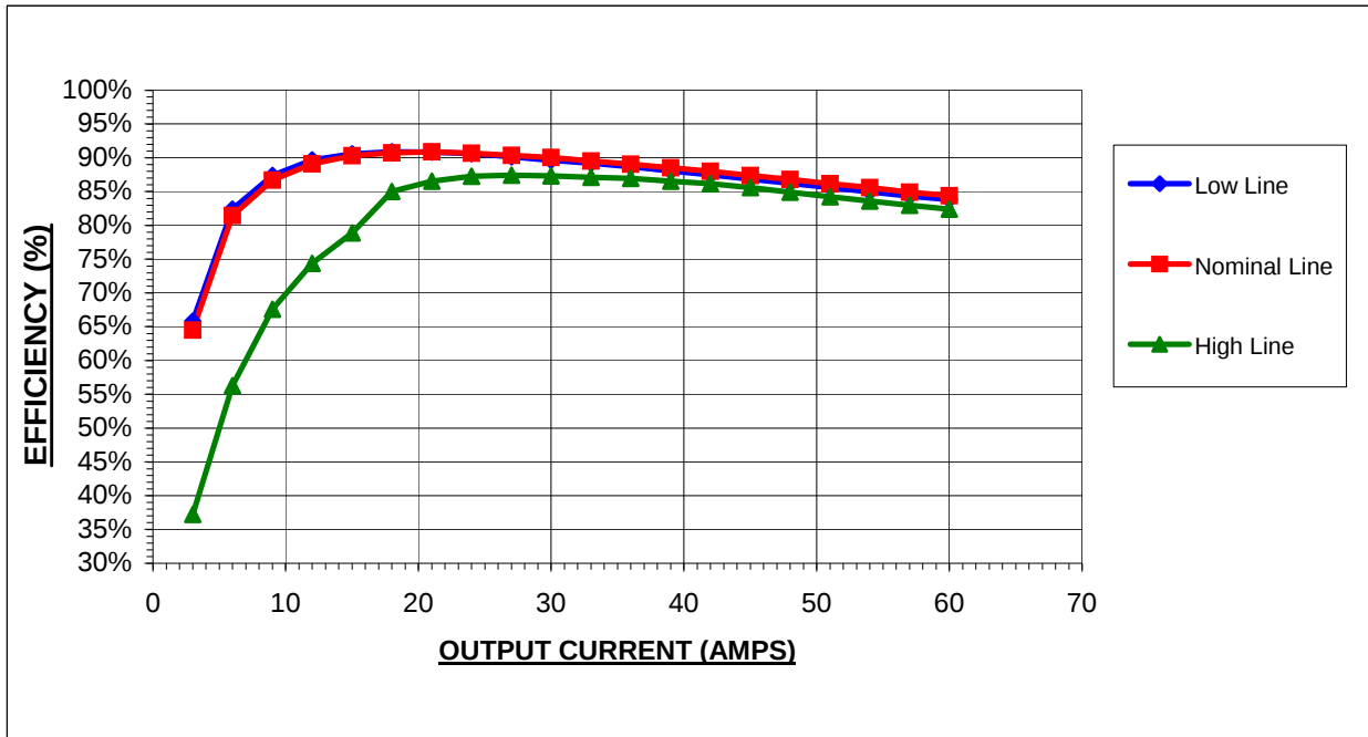
Graph 1: FA12S5-300 Efficiency vs. Output Current
