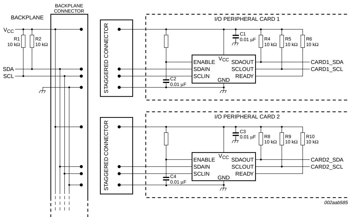
Fig 10. Hot swapping multiple I/O cards into a backplane using the PCA9514A in a PCI system
