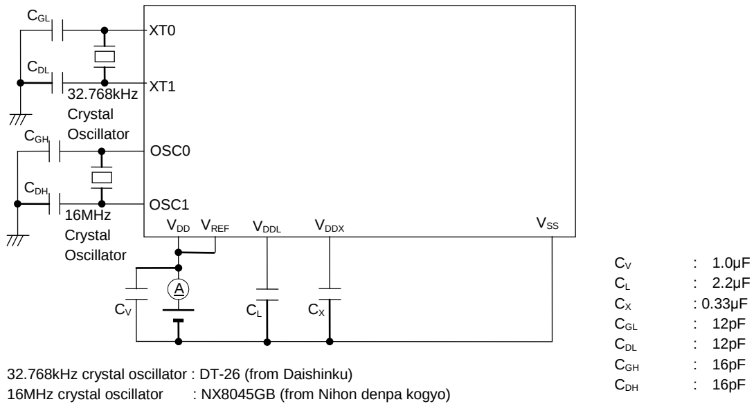
Measuring circuit 1
