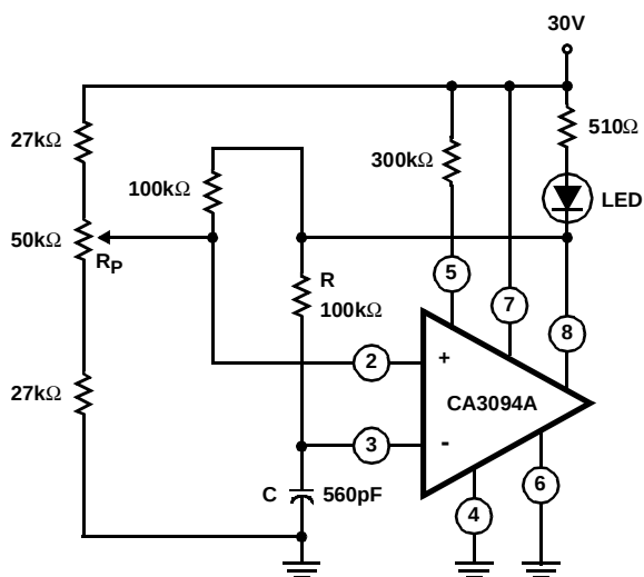
FIGURE 16. SINGLE SUPPLY ASTABLE MULTIVIBRATOR
