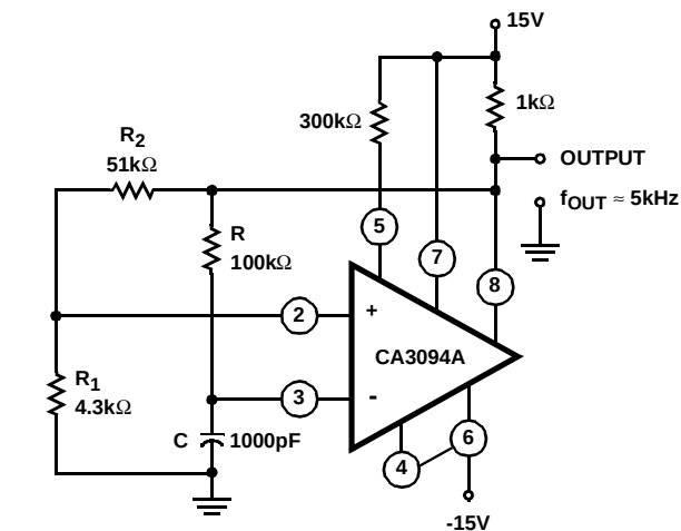
FIGURE 15. CURRENT OR VOLTAGE CONTROLLED OSCILLATOR
