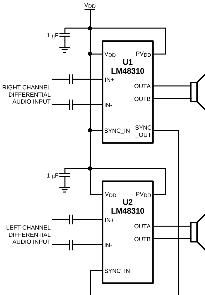
Figure 27. Cascaded LM48310
