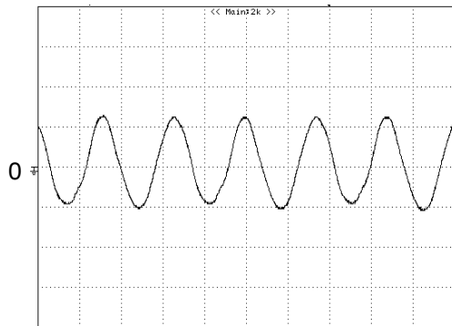
Figure 14: Output voltage ripple at nominal input voltage and rated load current ( I_o =full load)(50 mV/div, 1us/div)
