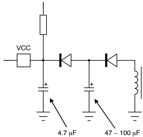
Figure 7. Split VCC Supply
