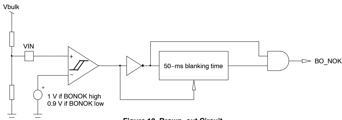
Figure 13. Brown-out Circuit
