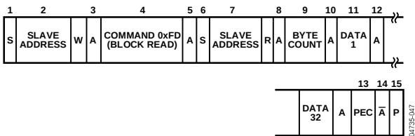
Figure 46. Block Read from EEPROM or RAM with PEC
