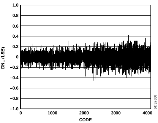
Figure 13. DNL for ADC
