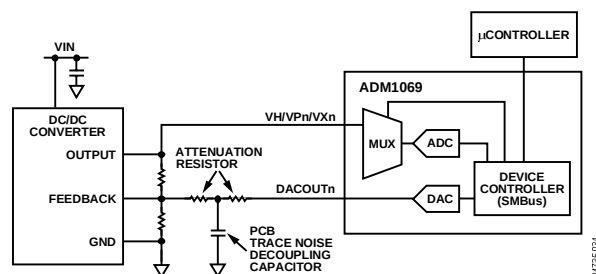
Figure 32. Closed-Loop Margining System Using the ADM1069
