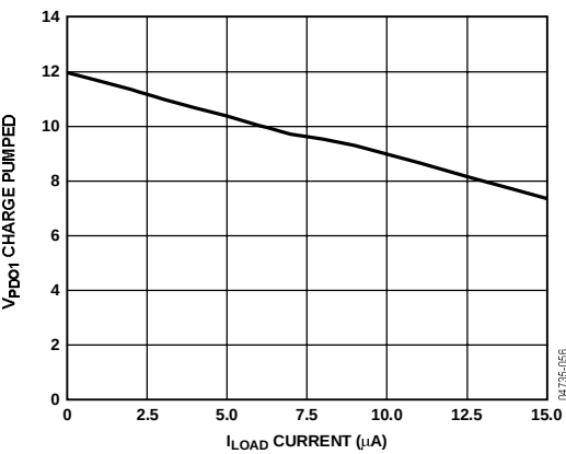
Figure 10. V_{PDO1} (FET Drive Mode) vs. I_{LOAD}
