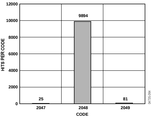
Figure 15. ADC Noise, Midcode Input, 10,000 Reads
