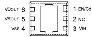
USP-6B (BOTTOM VIEW)
