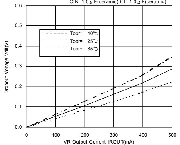
XC6402 Series (VR: 2.5V)
