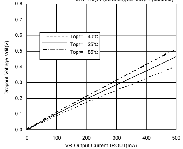
XC6402 Series (VR: 1.2V)
