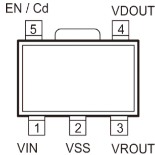
SOT-89-5 (TOP VIEW)
