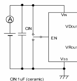
Circuit ②
