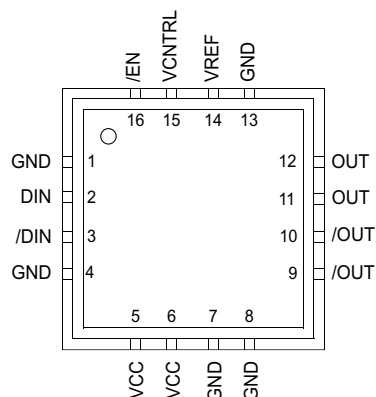
16-Pin MLF™
