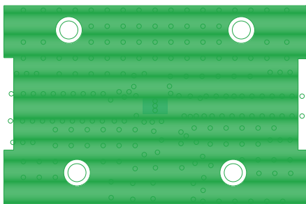
Layer 3: Ground
