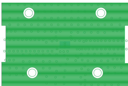
Layer 2: Ground
