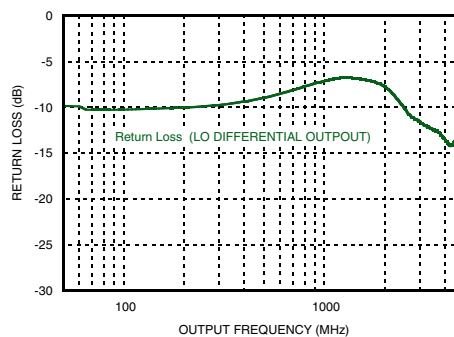
Figure 30. RF Output Return Loss Diff [21]
