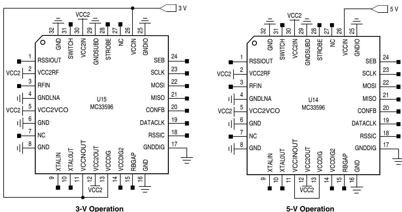
Figure 2. Wiring Diagrams
