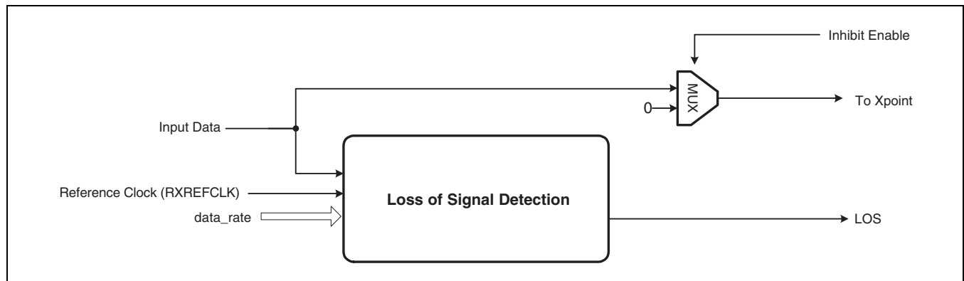
Figure 4-11. LOS Architecture
