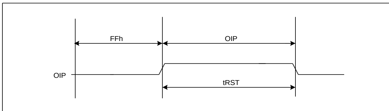
Figure20-4. Reset Timing
