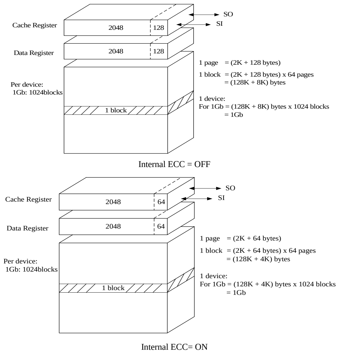
Figure3-1. Array Organization
