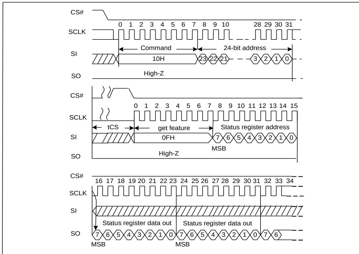
Figure11-3. Program Execute Sequence Diagram
