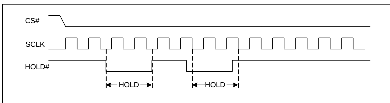
Figure5-2. Hold Condition
