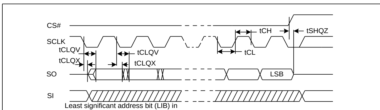
Figure20-2. Output Timing
