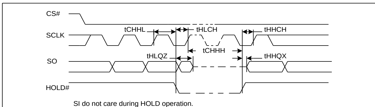
Figure20-3. Hold Timing
