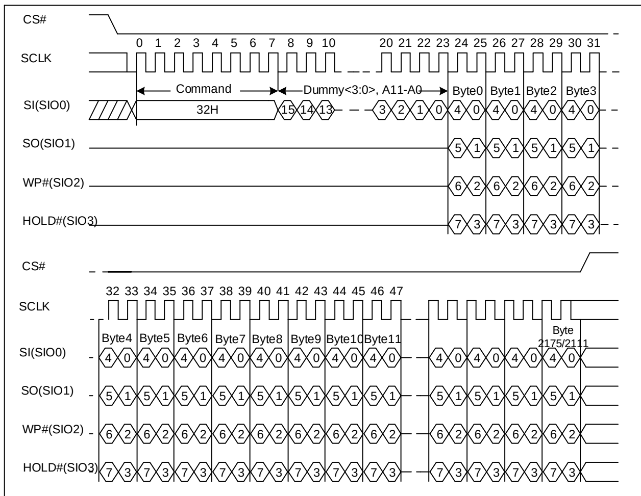
Figure11-2. Program Load x4 Sequence Diagram
