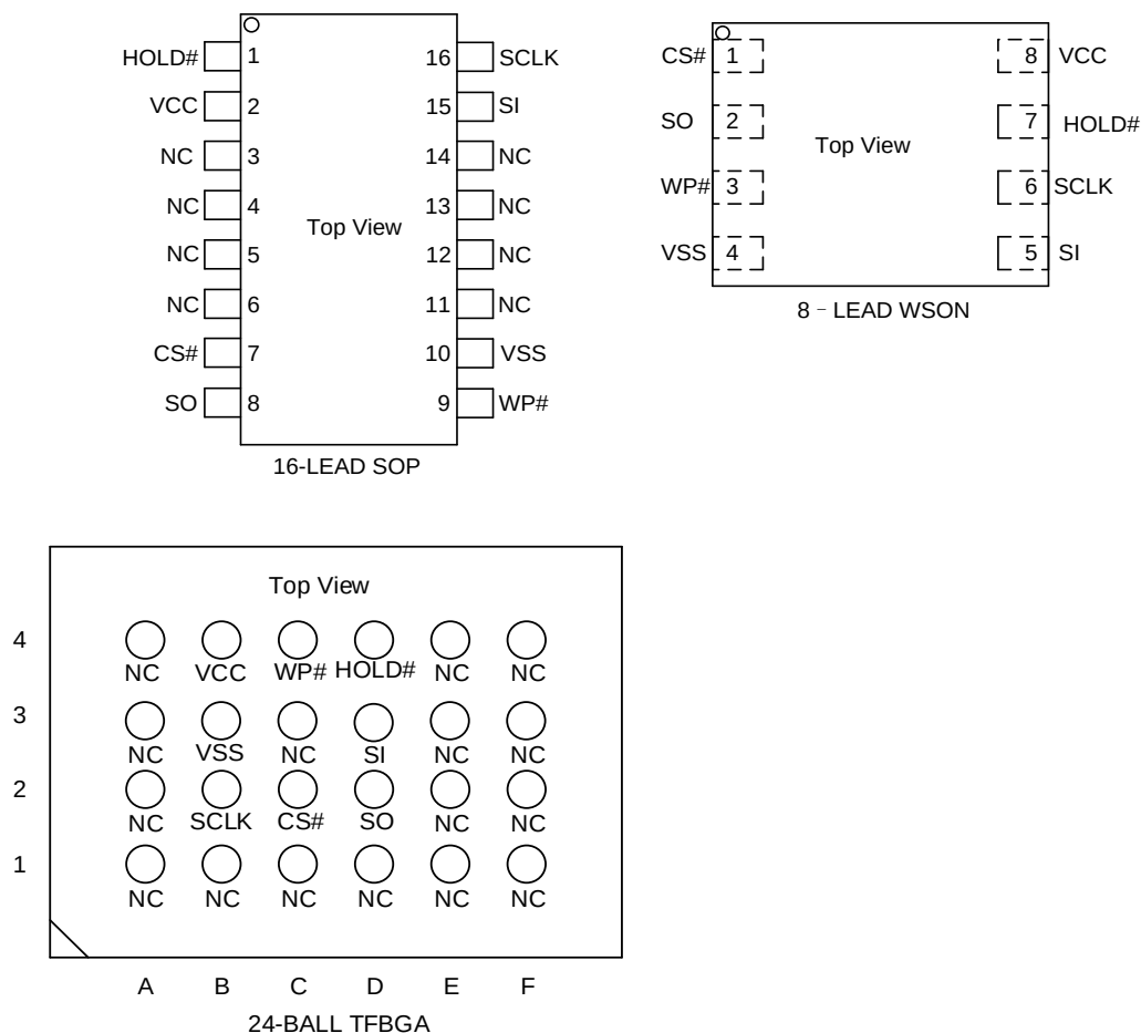
Figure2-1 Connection Diagram
