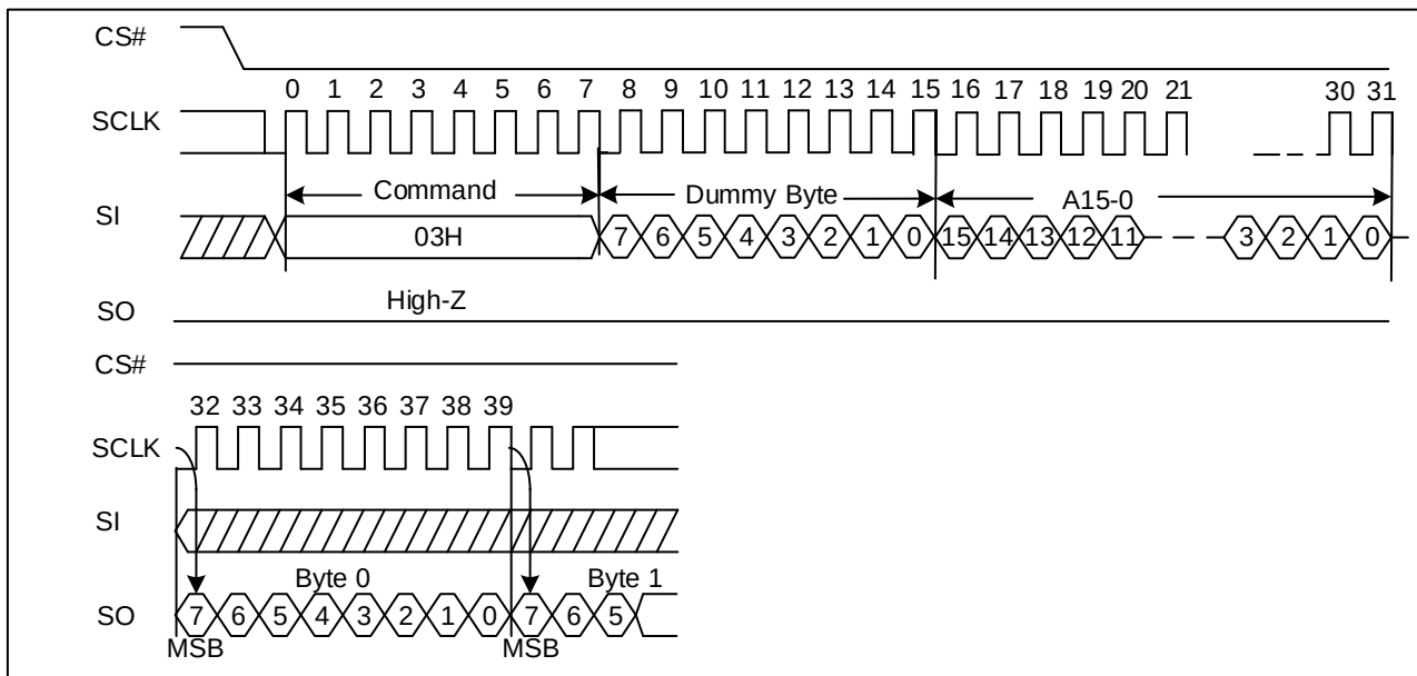
Figure9-2. Read From Cache Sequence Diagram
