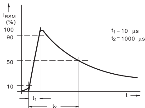
Figure5. Non-Repetitive Peak Reverse Current Pulse Definition
