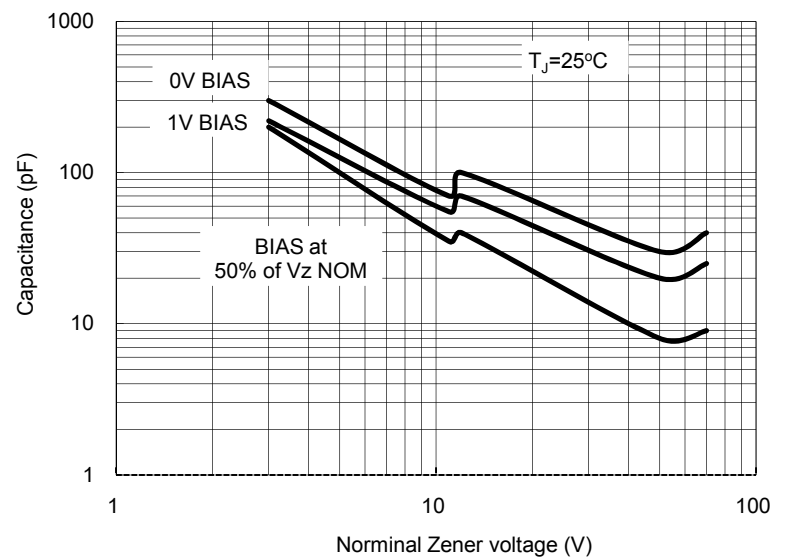
Fig. 4 Typical capacitance
