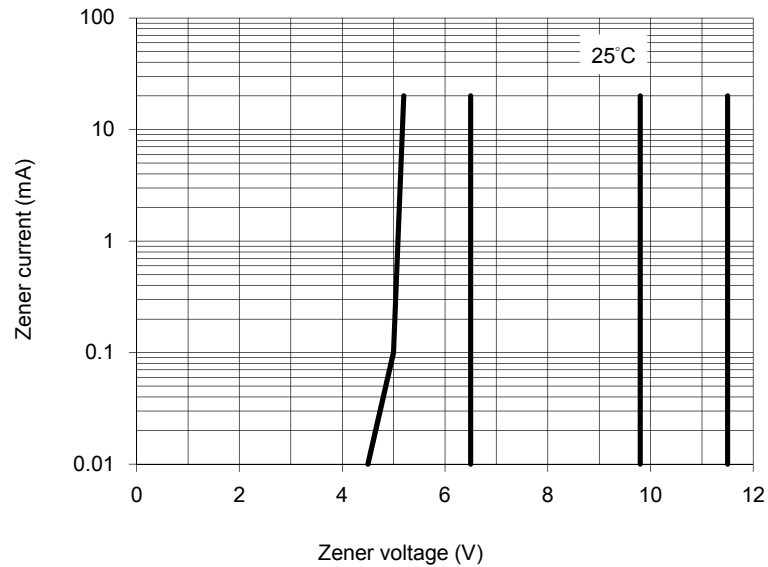
Fig.5 Zener breakdown characteristics
