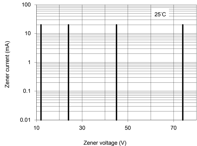
Fig.6 Zener breakdown characteristics
