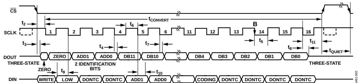
Figure 2. Gyroscope Serial Interface Timing Diagram
