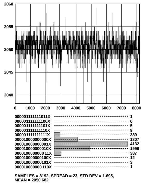
Figure 18. Noise Histogram
