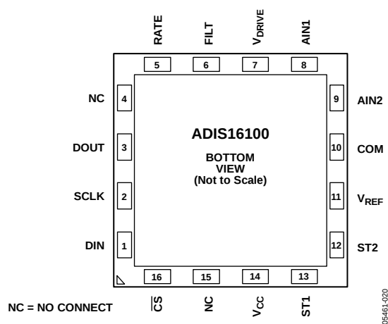
Figure 4. Pin Configuration
