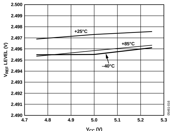
Figure 17. V REF vs. Supply Voltage
