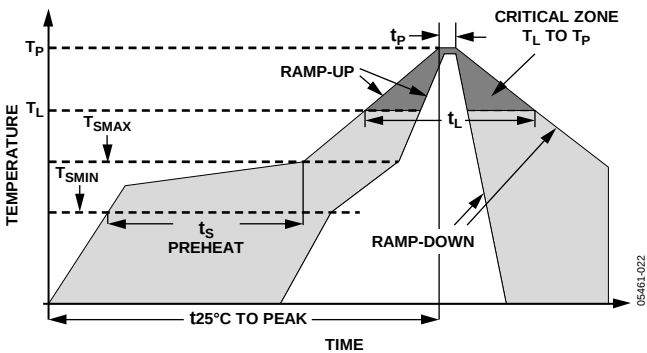
Figure 21. Recommended Solder Reflow Profiles
